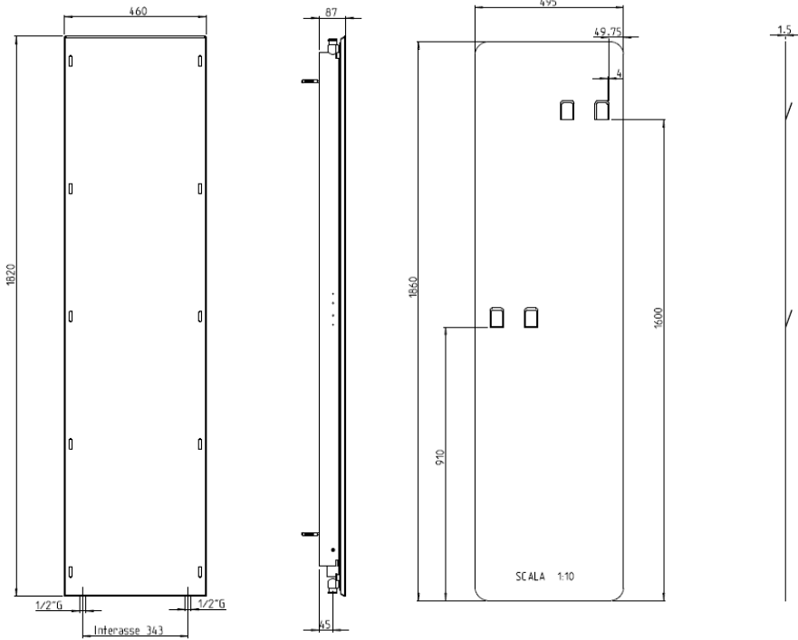
Body H = 1820 mm
